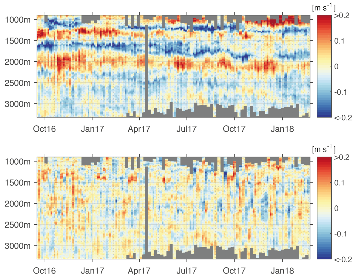
Fig. 2: Zonal (upper panel) and meridional velocity (lower panel) measured at the equator, 23°W with an MacLane profiler profiling up and down the mooring wire every six days. Note east- and westward current bands marked by red and blue colors, respectively, in the upper panel. The phase of these current bands slowly propagate downward, which is associated with upward energy propagation. The meridional velocity is dominated by monthly fluctuations most clearly visible at the end of 2017 (Fig. FPT).
